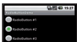
Fig. 9: RadioButton
