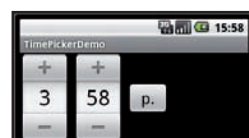
Fig. 12: TimePicker
